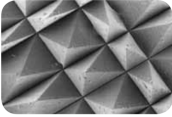
3M™ Trizact™ Abrasive surface, 50x magnification
